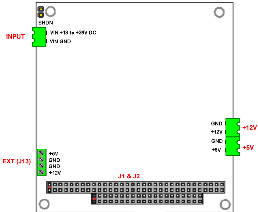
Figure 4. Connector layout
