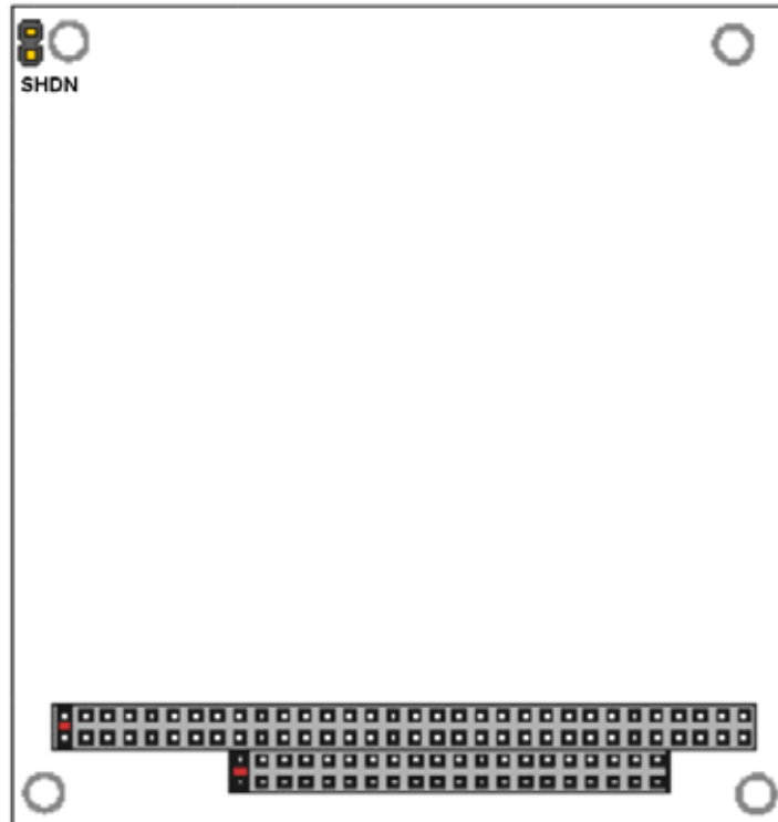
Figure 3. Jumpers and solder jumpers
